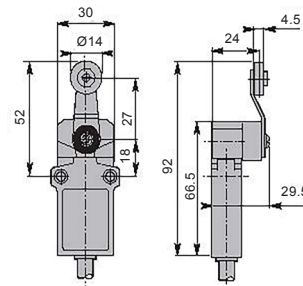
Roller lever
