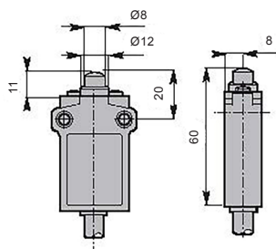
Plain plunger
