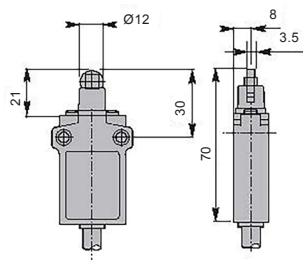
Roller plunger
